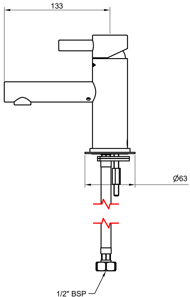
6230000RDX Mono Basin Mixer
