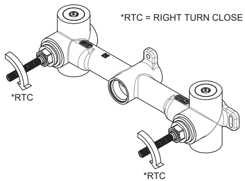
Part No: 5BMANIFOLDXH (Cross & Round Handles)
