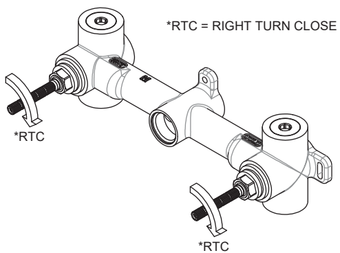
Part No: 5BMANIFOLDXH (Cross & Round Handles)
