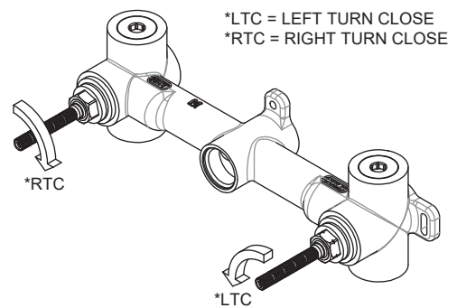
Part No: 5BMANIFOLDLV (Lever Handles)
